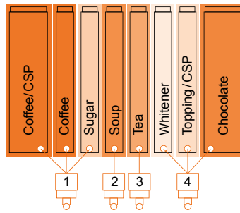
Variant 8401 B 8 product containers, 4 mixer units
