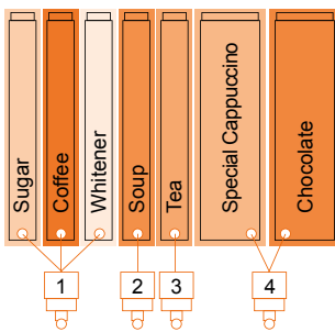
Variant 7401 7 product containers, 4 mixer units
